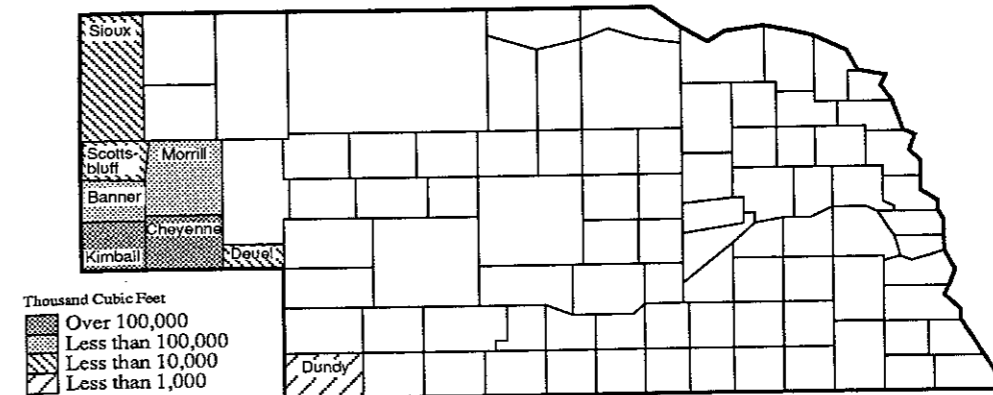
Figure 60 Production of Natural Gas by County, Nebraska, 1987
