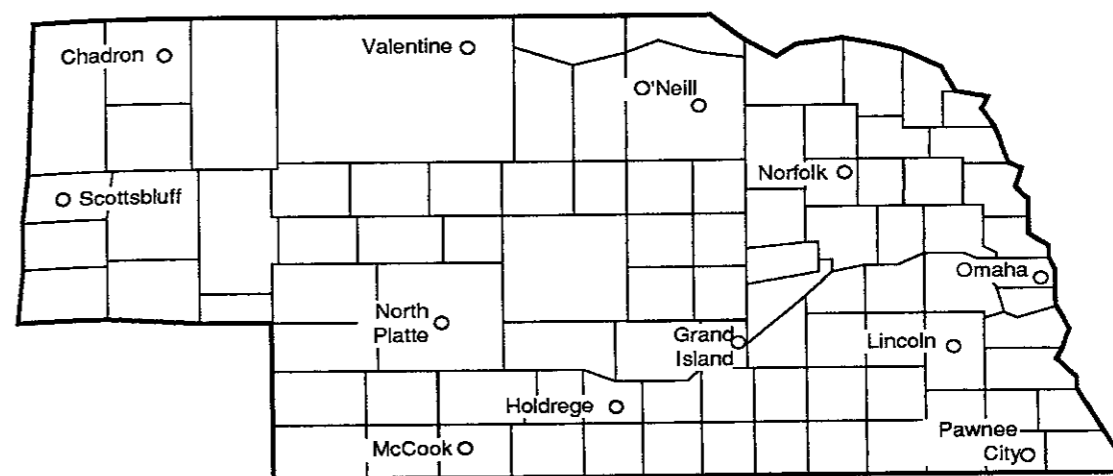
Figure 70 Nebraska Cities Represented in Charts VI-3 Through VI-14, Heating and Cooling Degree Days Monthly, 1975-1987 and Monthly Normals, 1951-1980
