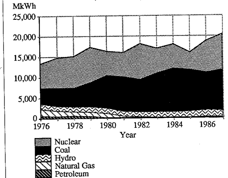
Figure 62 Electricity Generated by Fuel Type, Nebraska, 1976-1987 (Million Kilowatthours)
