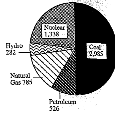
Figure 64 Operable Electric Generating Nameplate by Energy Source, Nebraska, 1987 (Megawatts)
